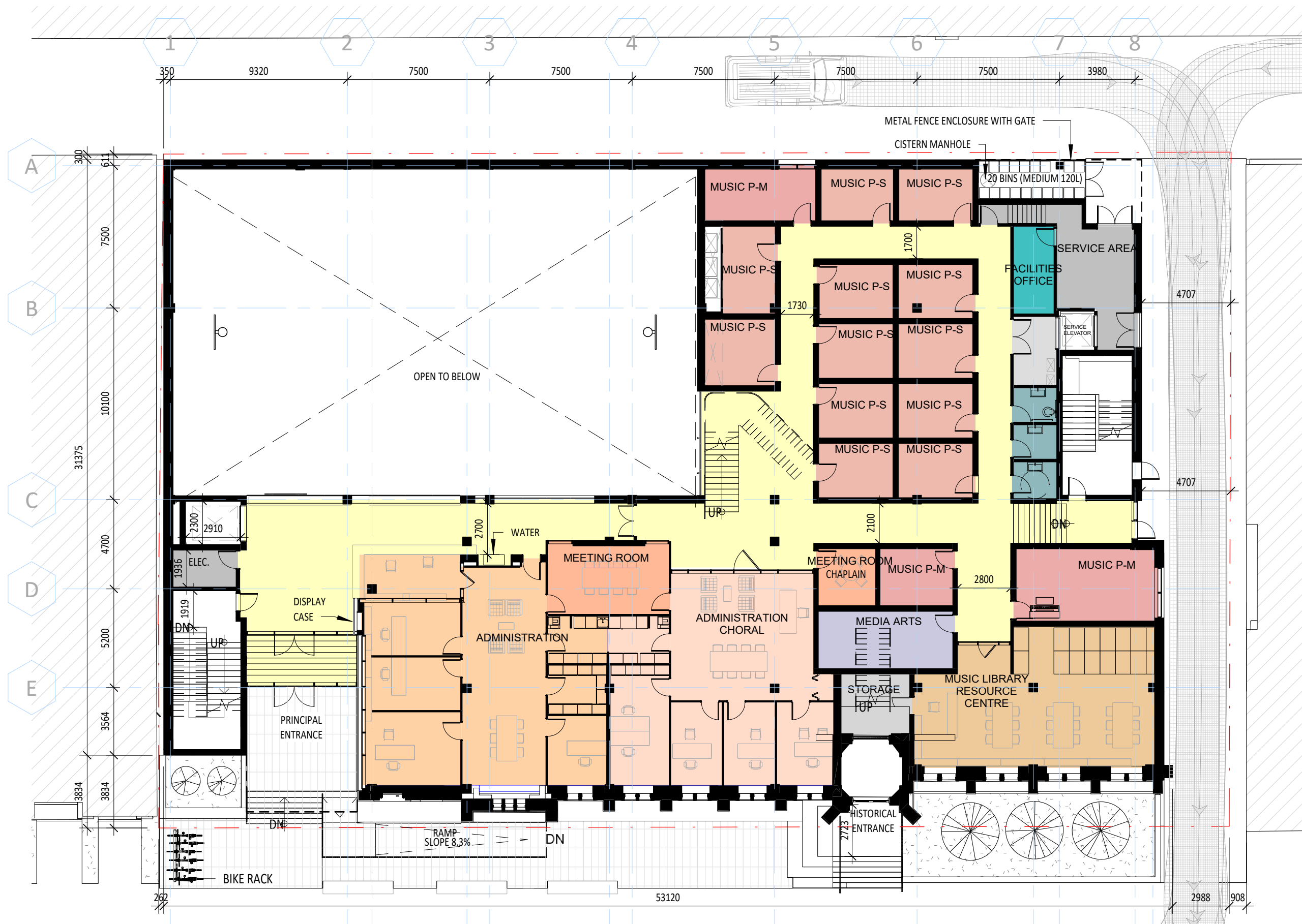
GROUND FLOOR ADMIN. & PRACTICE
